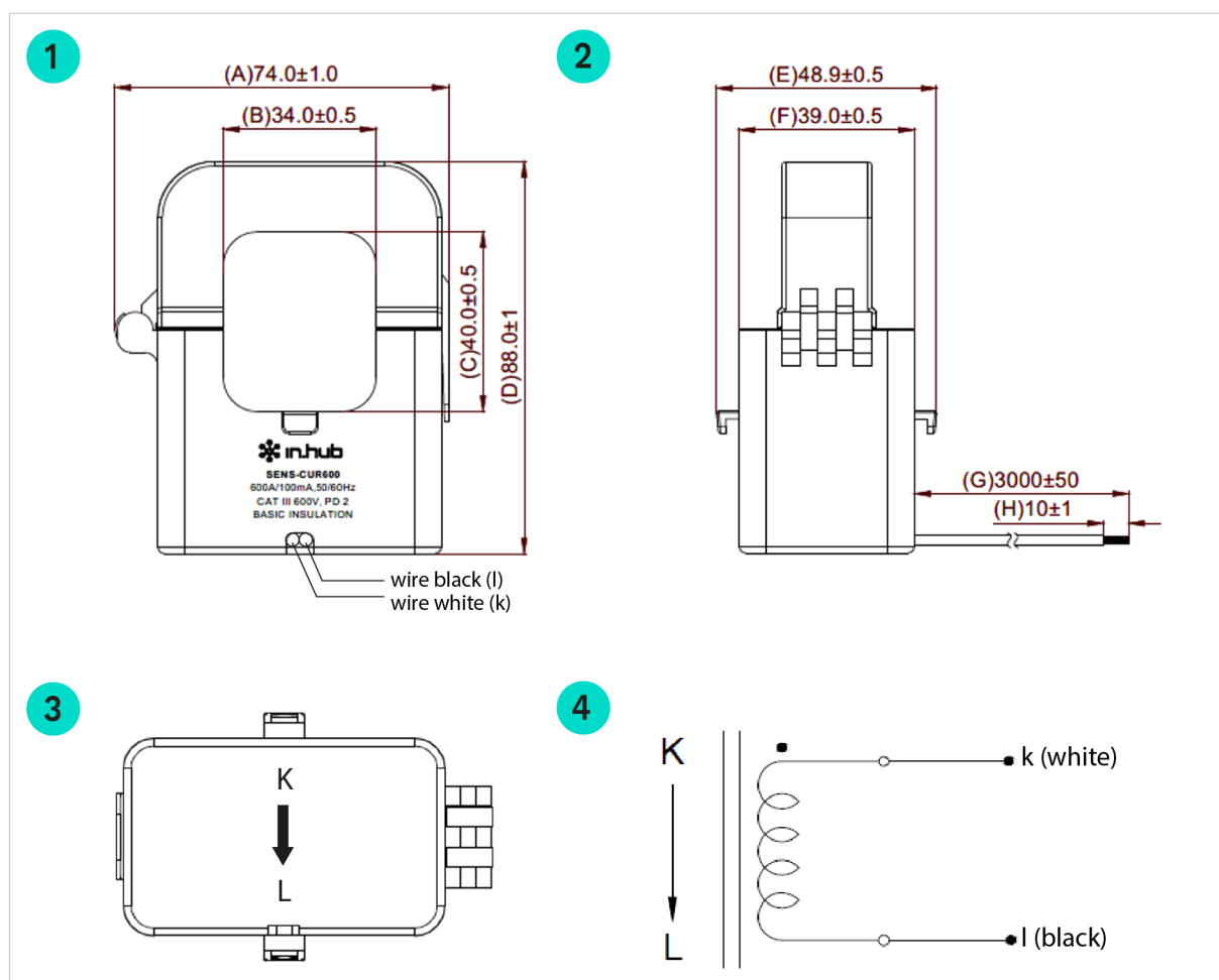
Dimensions of the SENS-CUR600 in mm
