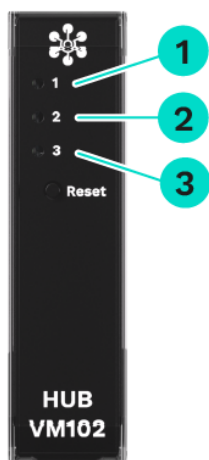
LEDs on the HUB-VM102
